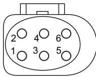
6 pins Bosch female connector front view
