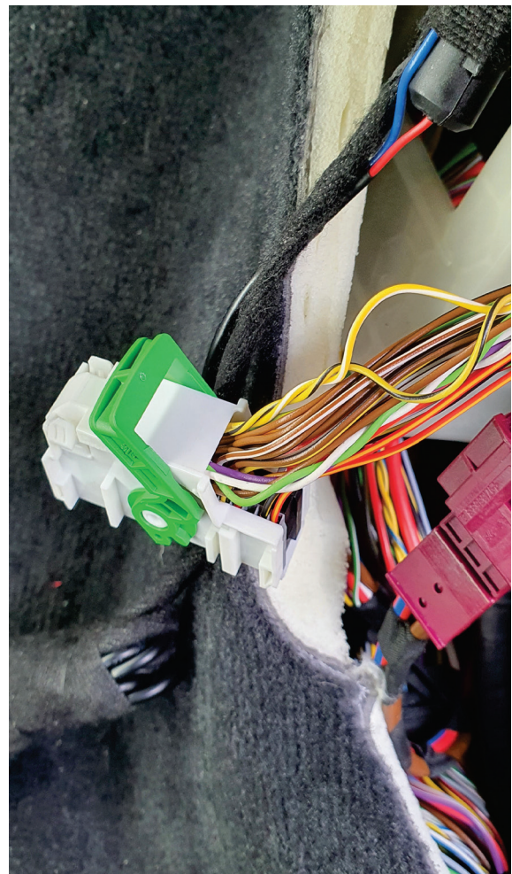
AIM cable CAN + CAN -
