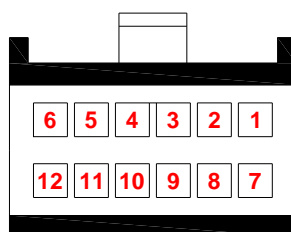
AMP 12 pins female connector pinout Contact insertion view
